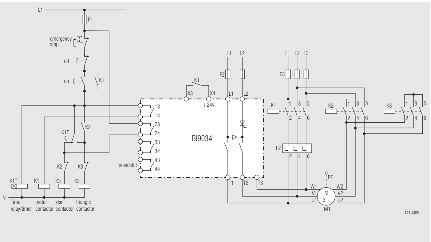
BI 9034 with external star-delta-control
